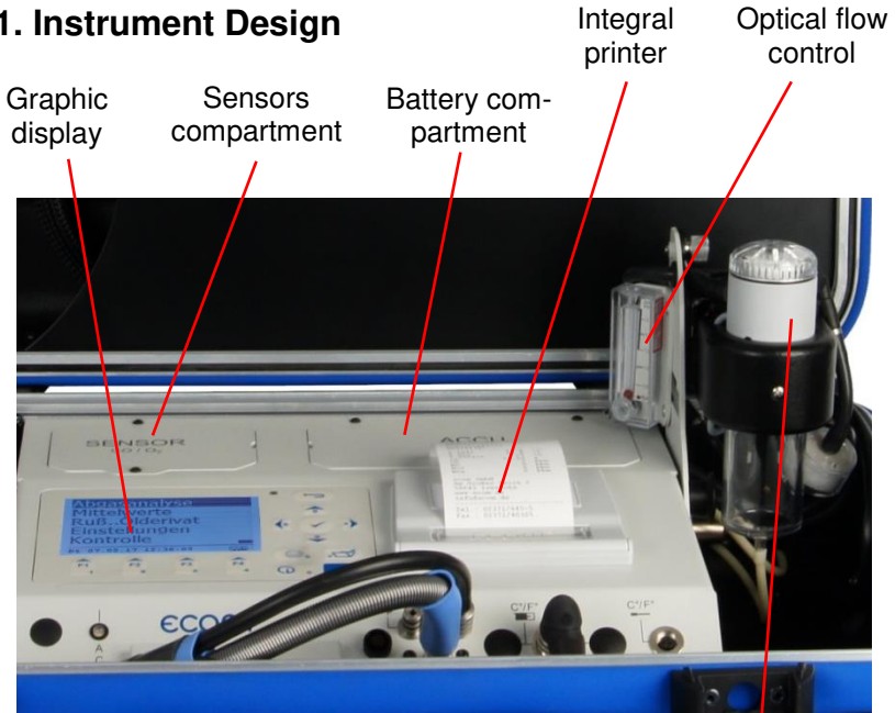
Condensation trap (with peltier cooler) with fine dust filter
