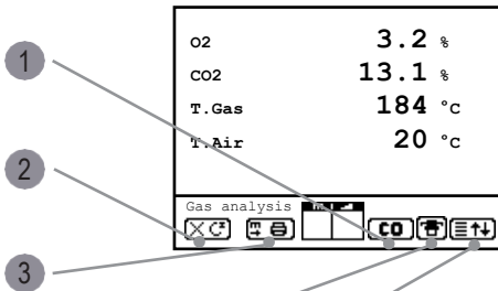
Measurement display: Gas analysis 1 + 2
